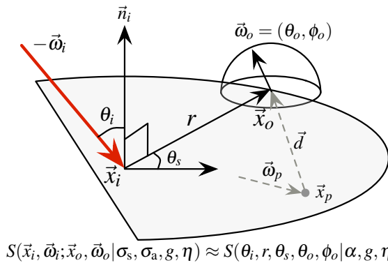
Figure 2: Geometric setup for our simulation and model. A collimated beam of light arriving at point \vec{x}_i from direction \vec{\omega}_i (shown in red) makes angle \theta_i with the surface normal. A photon from this beam that arrives at point \vec{x}_p propagating in direction \vec{\omega}_p has an exitant trajectory \vec{d} towards the point \vec{x}_o = (r, \theta_o) on the surface. This particular photon path exits the material in direction \vec{\omega}_o = (\theta_o, \phi_o) .
